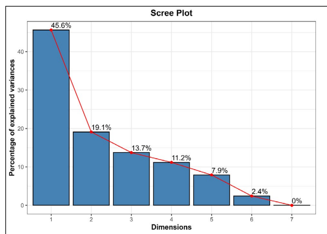
Figure 3: Scree plot showing the percentage of variance explained by each principal component
